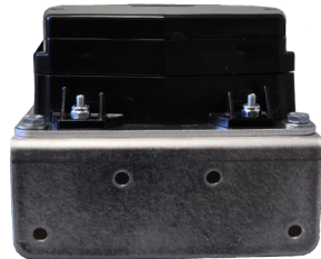
BT-3000 WITH MOUNTING PLATE AND BRACKET
